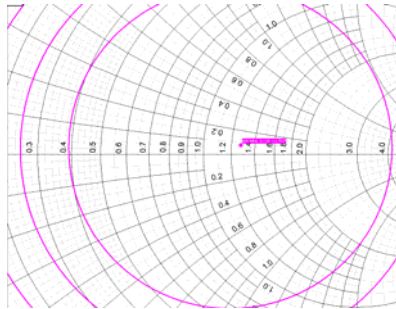
Noise Circles
